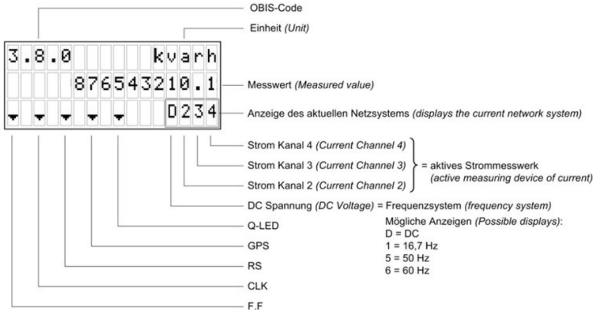
Figure 4.1: LC display
