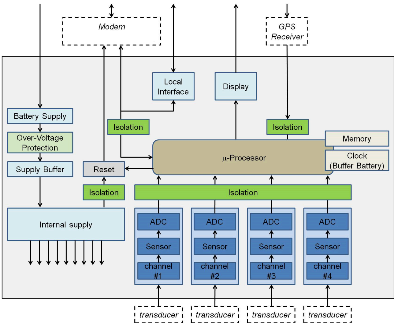
Figure 2.1: Block diagram
