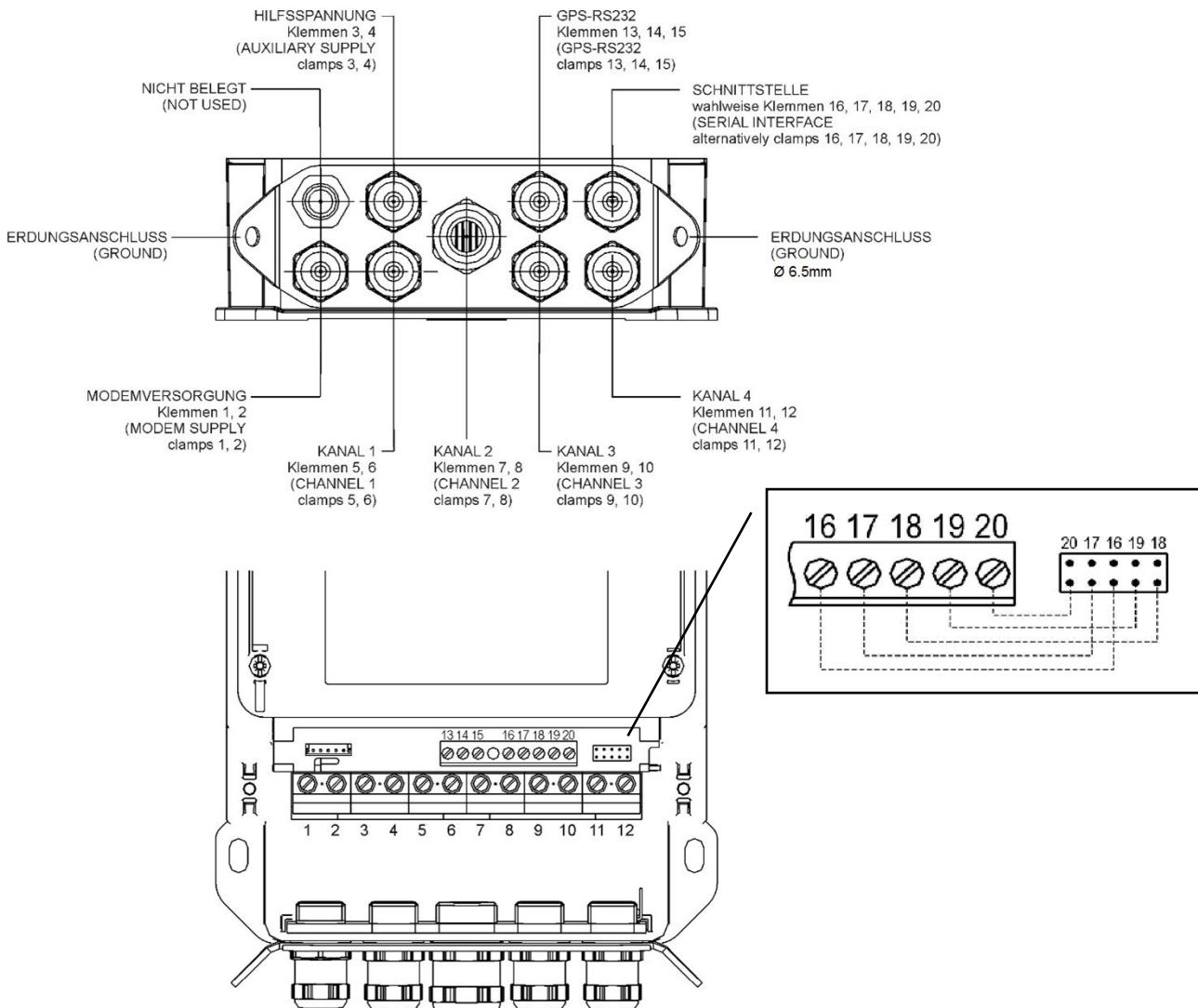
Figure 3.2: Terminal block
