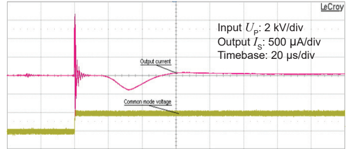
Figure 14: Detail of typical common mode perturbation (2000 V step with 6 kV/µs, R_M = 100 \Omega )
