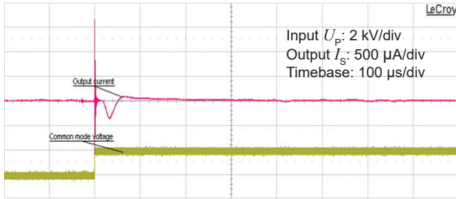
Figure 13: Typical common mode perturbation (2000 V step with 6 kV/µs R_M = 100 \Omega )
